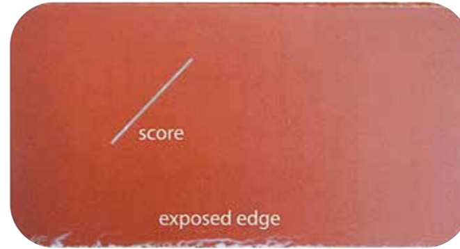
The pictured sample was the result of 500hrs Salt Spray Test ASTM B117. Minor oxidisation was observed at the exposed edge.
